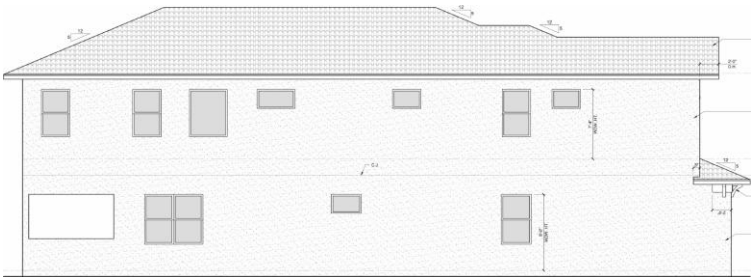
Left Elevation
